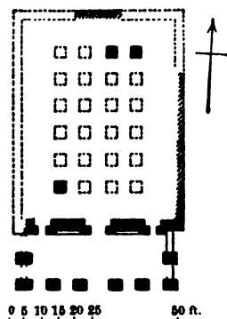
Synagogue at Kefr Bir'im in Galilee (Ground-Plan).
